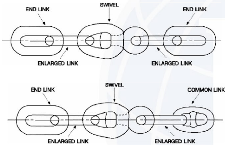
Typical Swivel Assemblies
